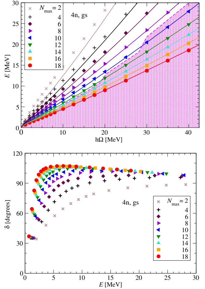
FIG. 1. NCSM results for the tetra-neutron ground state energy obtained with various N_{\max} (symbols) plotted as functions of \hbar\Omega (upper panel). The shaded area shows the NCSM result selection for the S -matrix parametrization; the solid curves are obtained from the phase shifts parametrized with a single resonance pole by solving Eq. (2) for the eigenenergies at given N_{\max} and \hbar\Omega values. The 4 \rightarrow 4 phase shifts obtained directly from the NCSM results using Eq. (2) are shown in the lower panel.
